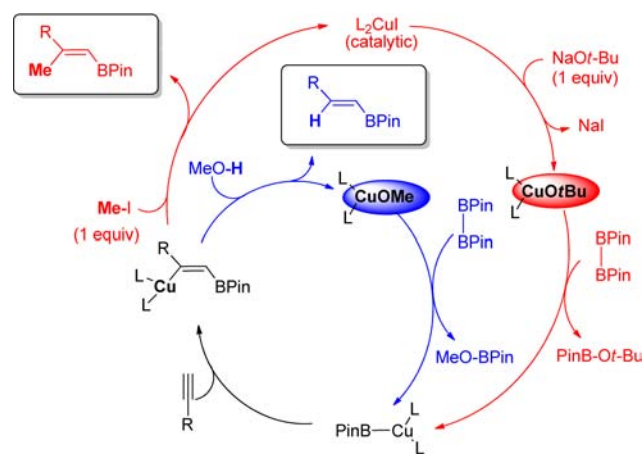
Scheme 2. Comparison of the Catalytic Cycles of the Cu-Catalyzed Hydroboration and Carboboration (Present Work)
